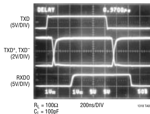
Driver Output Waveforms
