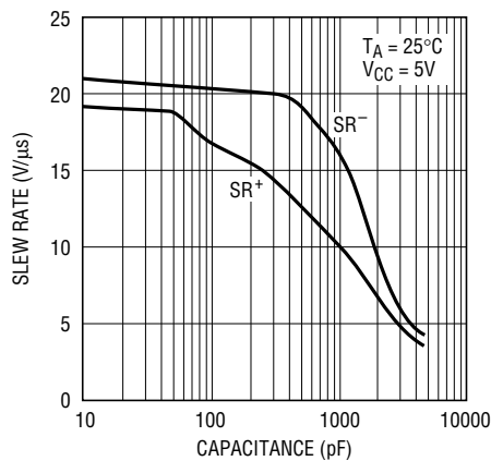
RS232 Driver Slew Rate vs Load Capacitance
